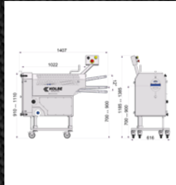
PORTIOMAT PM150
